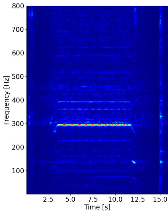
(a) up-drive condition, Elevator 4
