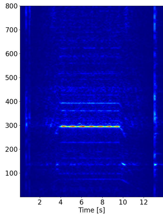
(b) down-drive condition, Elevator 4
