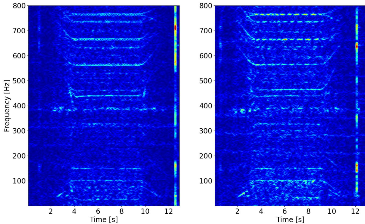
(c) up-drive condition, Elevator 1
